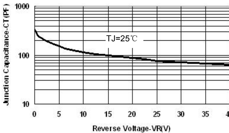
Fig.1-Typical Junction Capacitance
