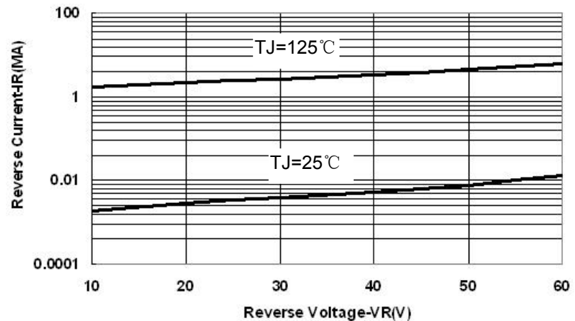
Fig.2-Typical Reverse Characteristics
